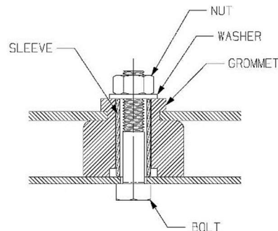
Figure 1 – Typical Assembly of Mounting Hardware
