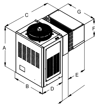
cold room hole opening dimension
